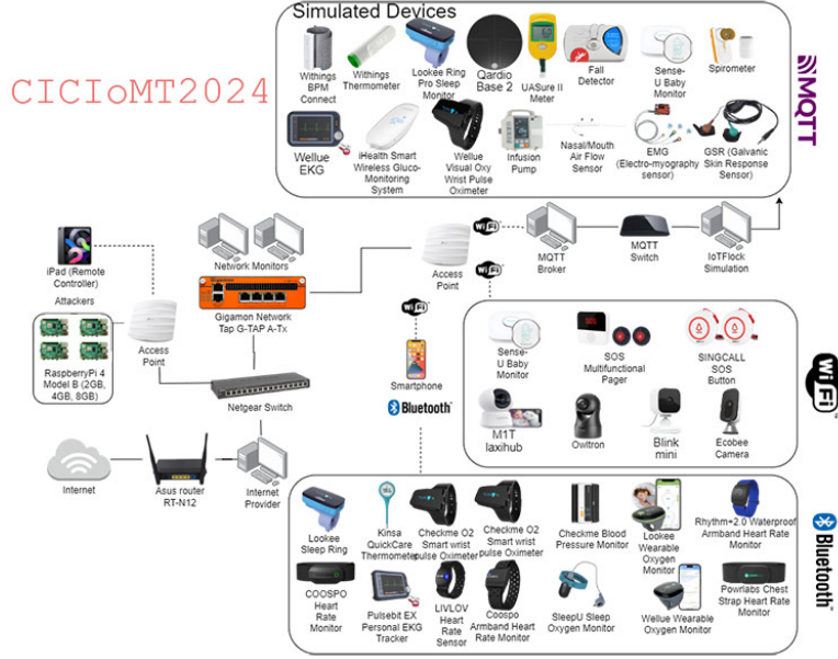
Figure 2: CICIoMT2024 topology. Source: [3]
